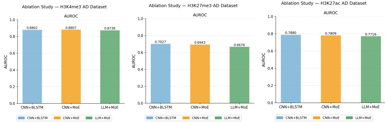
AUROC of three reproduced models across 3 histone modifications in AD dataset
